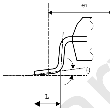
Detail F
